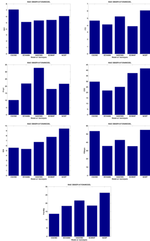
Figure 10. Same as Figure 9 but for the mean spatial MAE.
