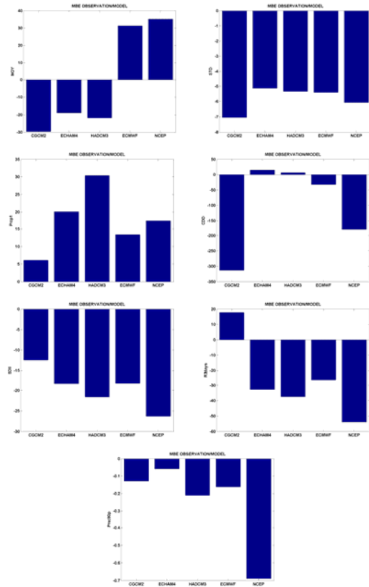
Figure 9. Mean spatial MBE values for each indice from GCMs/reanalyses over April-October and 1961-1990. For each indice (names given in y-axis), MBE is given for CGCM2, ECHAM4, HadCM3, ECMWF and NCEP, respectively, from left to right.
