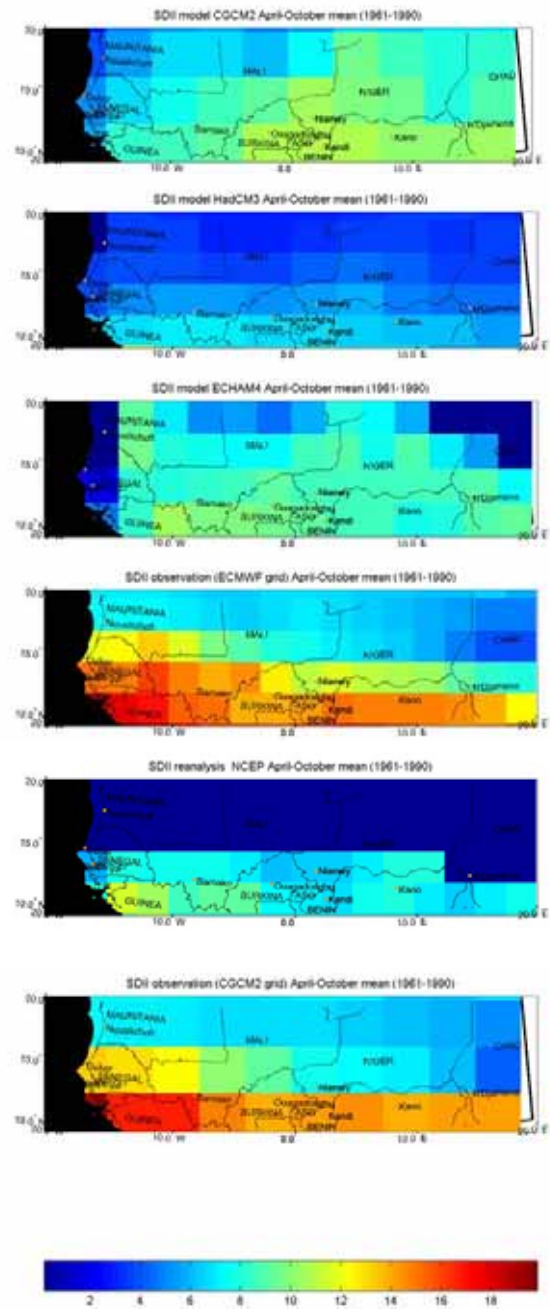
Figure 5. Same as Figure 2 for the simple daily precipitation index SDII (in mm/day).
