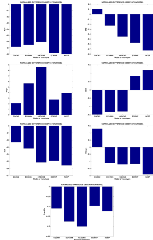
Figure 11. Same as Figure 9 but for the mean spatial ND (normalized values).
