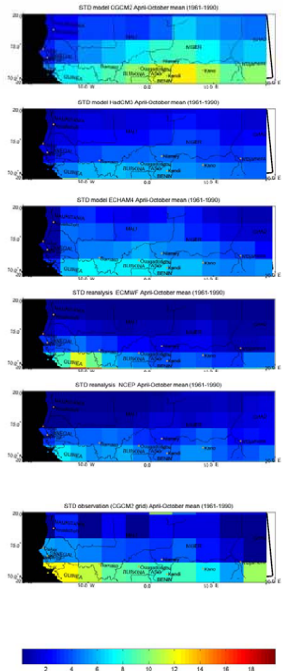
Figure 3. Same as Figure 2 for the intra-seasonal standard deviation simple (in mm/day).
